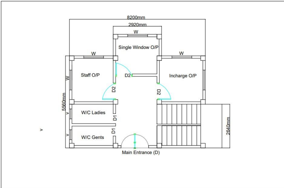
Ground Floor Plan Of Proposed Police Outpost at Deorali, Gangtok East Sikkim.
